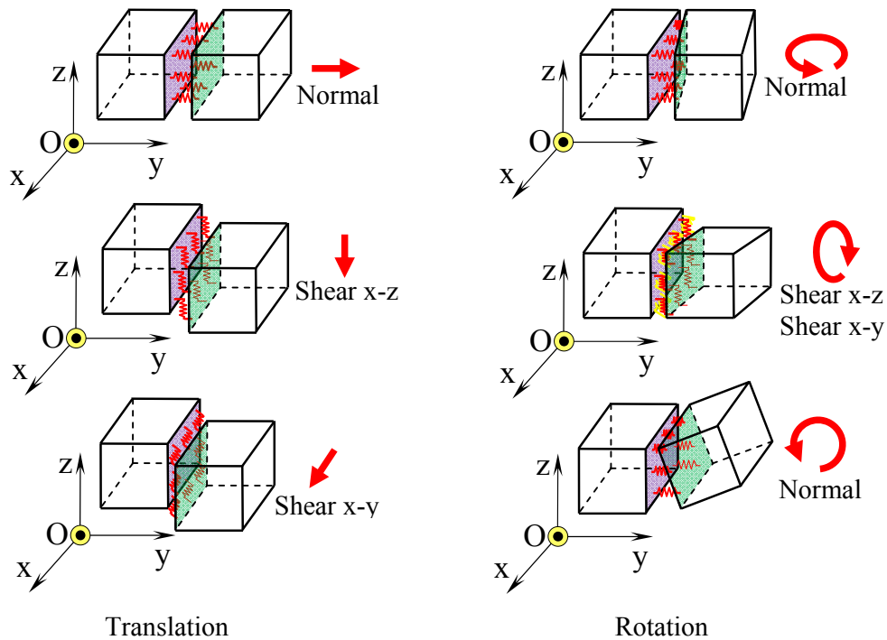
Figure 2. The attached springs
