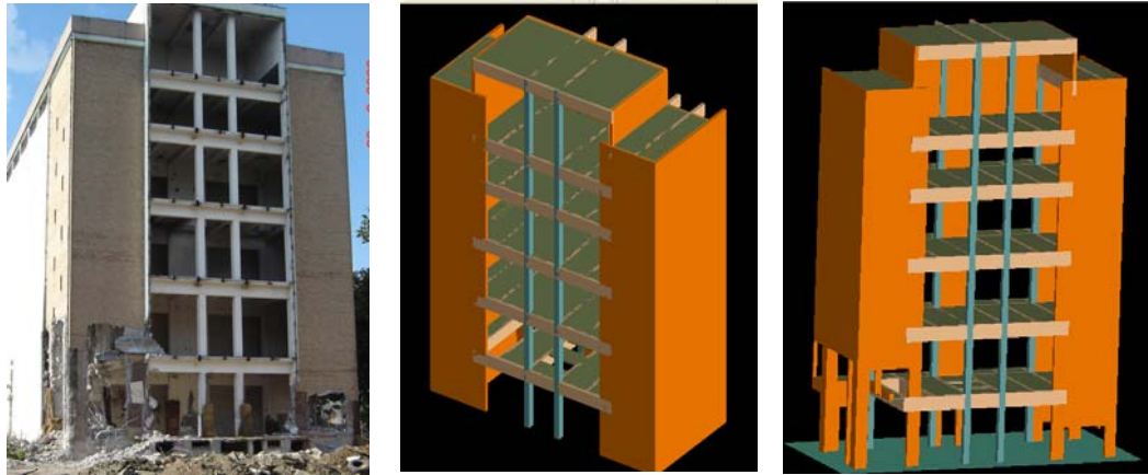
Figure 6. Real and simulated structure before demolition: a) real construction after preparatory works; b) geometrical model of structure; c) geometrical model of structure before starting simulation.
