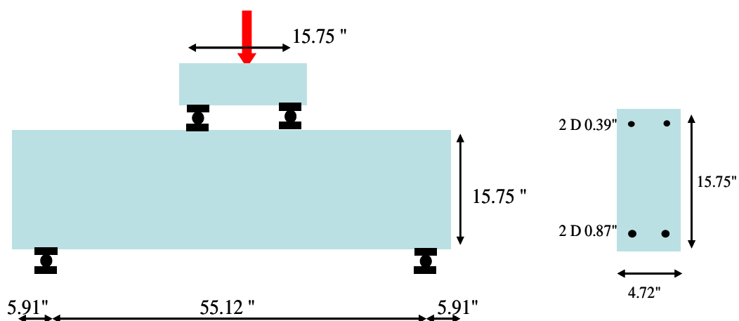
Fig. 1.a Problem geometry
