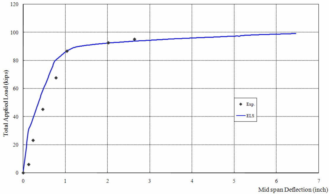
Fig. 2 Load-deflection predicted by ELS in a comparison to the experimental results
