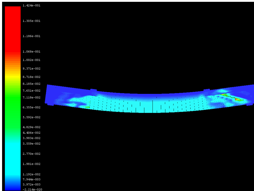
Fig.3 Principal strain contours (in 1_Dir) at applied load -99.126 kip (at output frame 411) predicted by ELS
