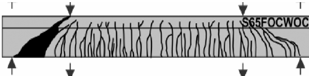
Fig. 4 Observed experimental cracking pattern
