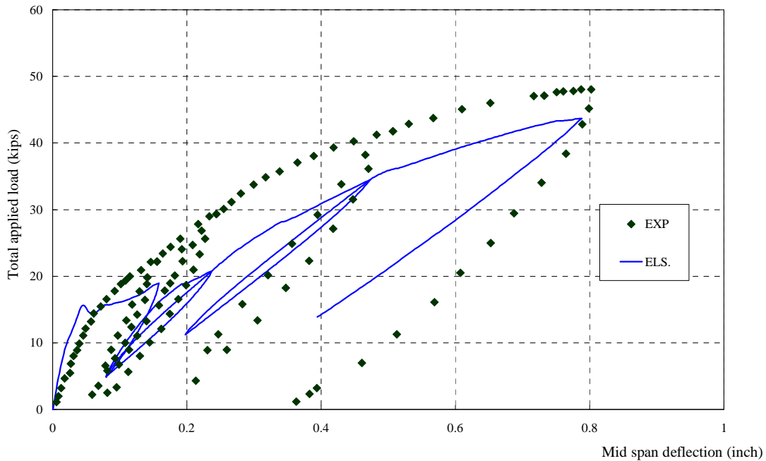
Fig. 1 Load-deflection predicted by ELS in a comparison to the experimental results
