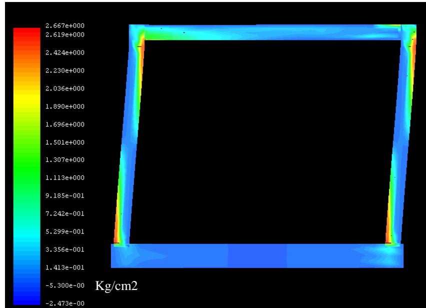
Fig. 2.a Normal stress in x-direction.
