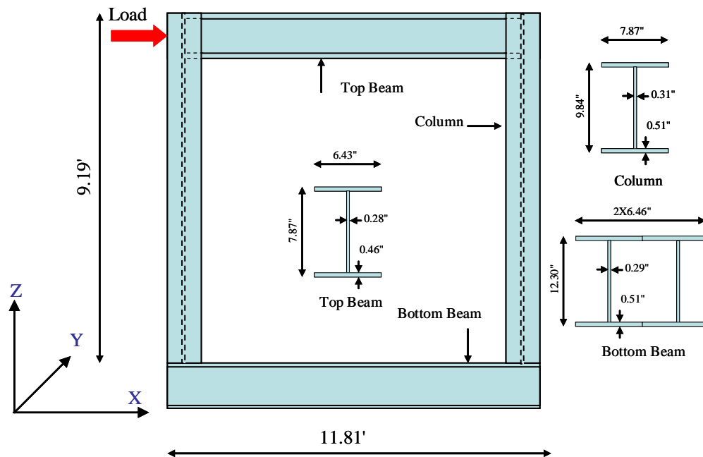
Fig. 1.a Problem geometry.
