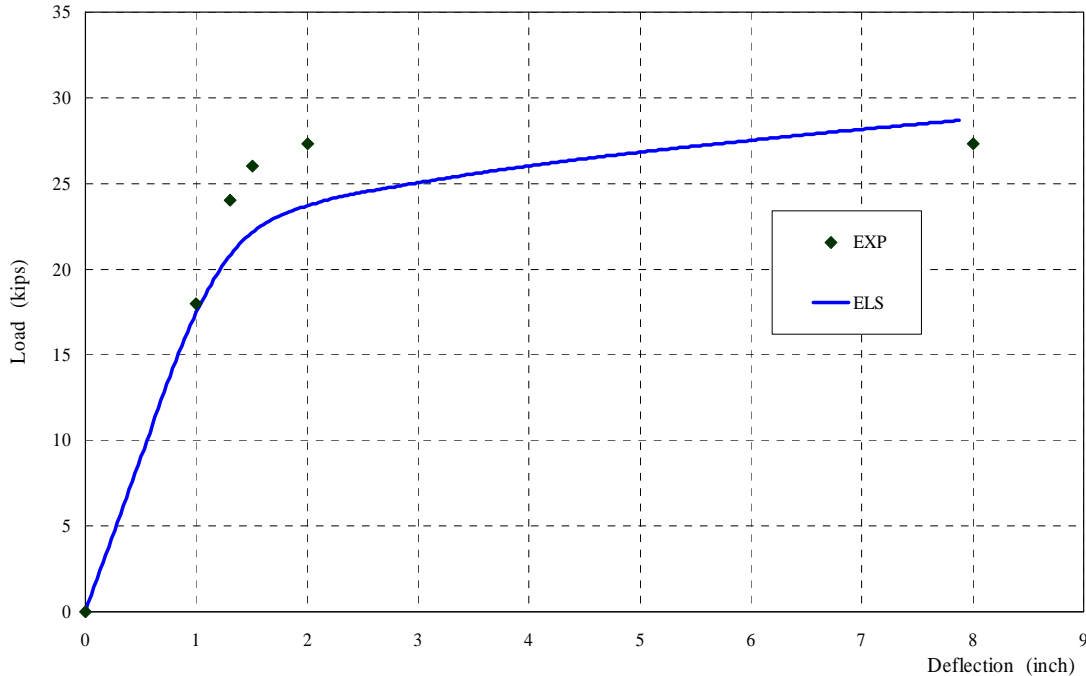
Fig. 3 Load-displacement curves comparison between ELS® and experimental data.
