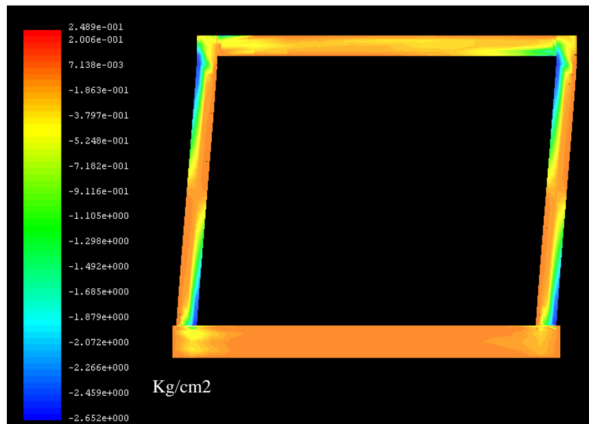
Fig. 2.b Normal stress in z-direction.
